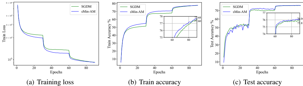
Figure 2: Experiment of training ResNet50 on ImageNet.
