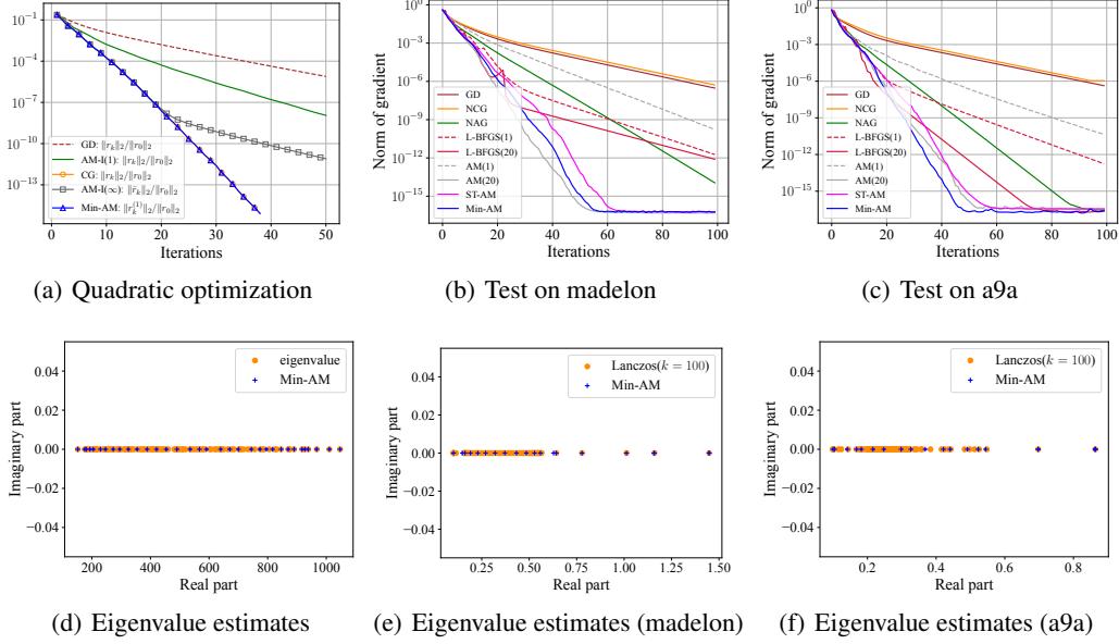
Figure 1: Left (strongly convex quadratic optimization): (a) curves about residuals and intermediate residuals; (d) exact eigenvalues, and eigenvalue estimates from Min-AM. Middle and right (regularized logistic regression on madelon and a9a datasets): (b)(c) \|\nabla f(x_k)\|_2 of each method; (e)(f) Ritz values of \nabla^2 f(x^*) by k -step Lanczos algorithm, and eigenvalue estimates from Min-AM.
